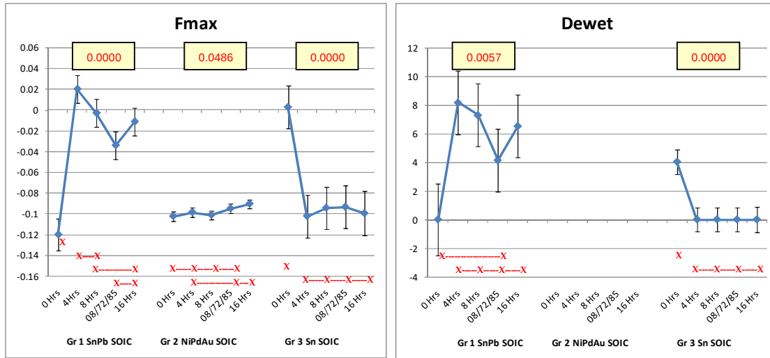
Figure 4 – Experiment 1 test results for Groups 1 to 3, the SOIC packages - (Top Yellow Boxes show ANOVA p-values, the bottom red X's and connecting lines illustrate which averages are close enough to be considered "not significantly different" in these results.) Graph shows average and 95% confidence interval.
