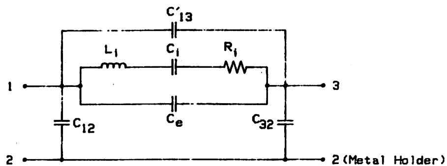
EQUIVALENT CIRCUIT
