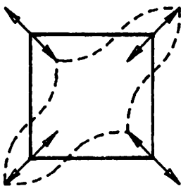
FACE SHEAR
