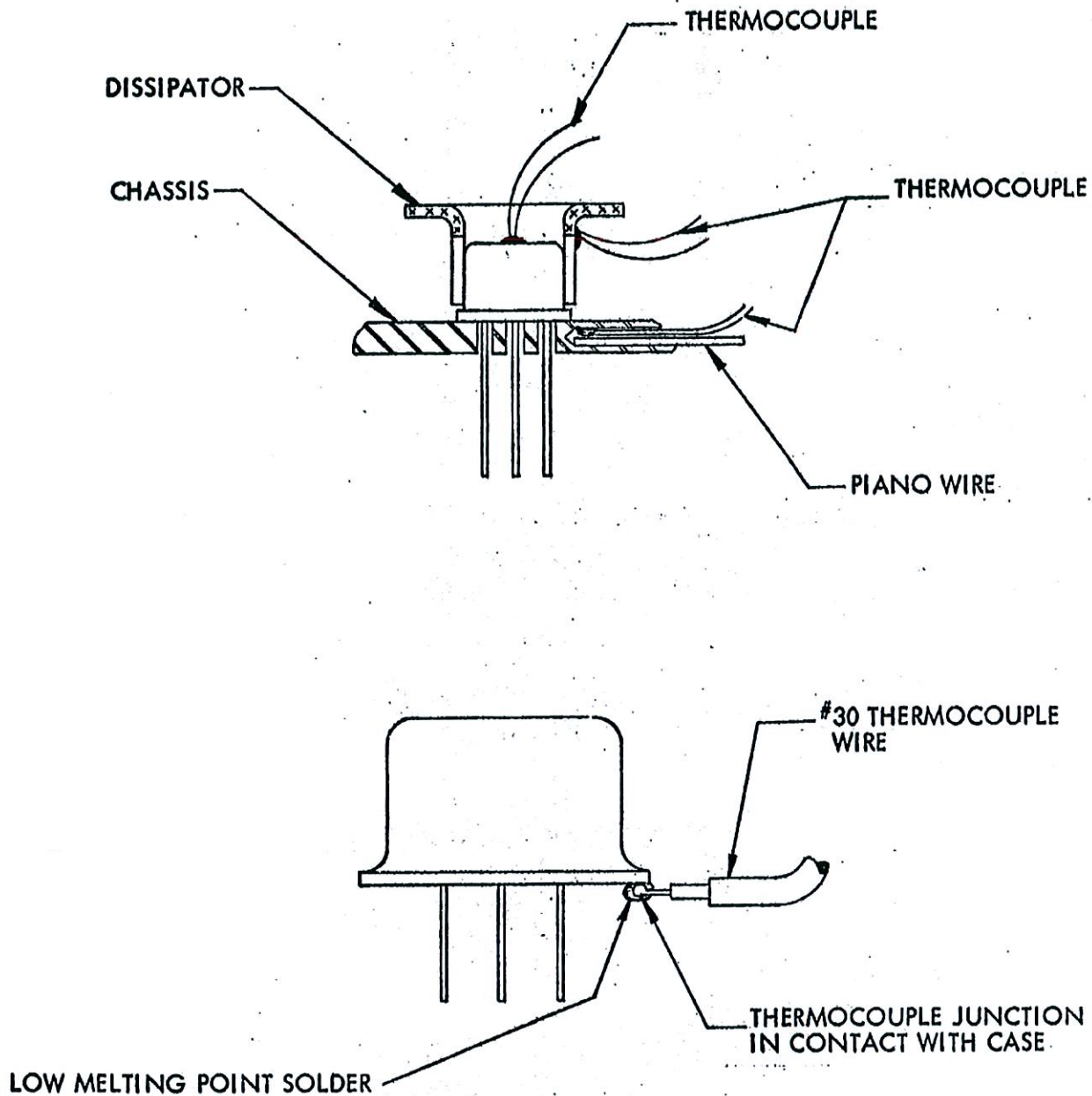
THERMOCOUPLE ATTACHMENT FOR NON-STUD TYPE TRANSISTOR WITH METAL BASE TOO THIN FOR MOUNTING IN FLANGE
