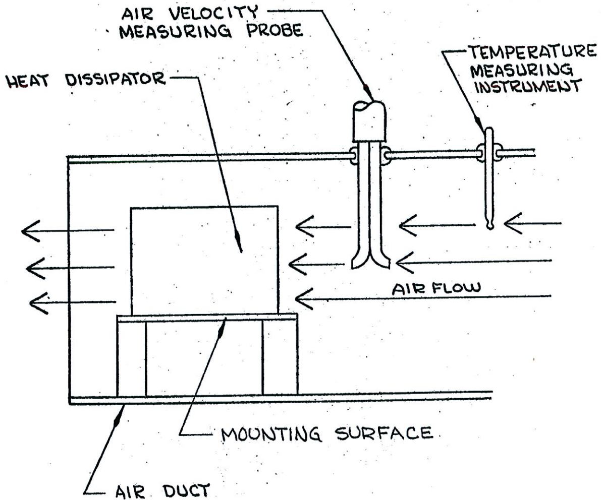
FIGURE 10 FORCED AIR MEASUREMENT, LINEAR
