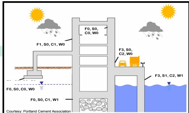
Durability Exposure Classes for Concrete Members
