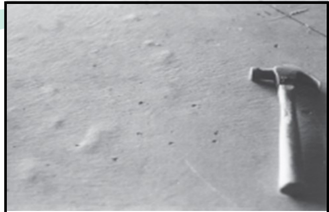
BLISTERS ON CONCRETE SLAB
