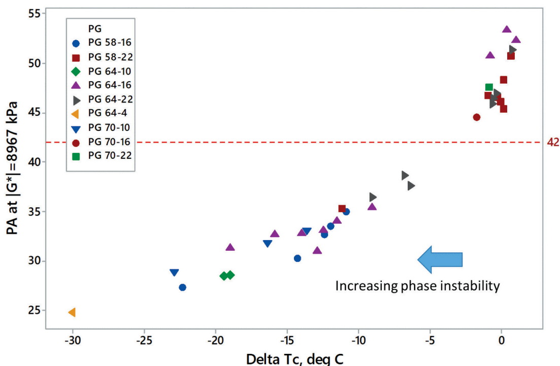
Figure 33. Relationship Between \Delta T_c and Phase Angle at Intermediate Temperatures (23)
