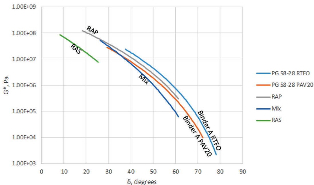
Figure 28. Black Space Curves from Bullitt County Project (22)
